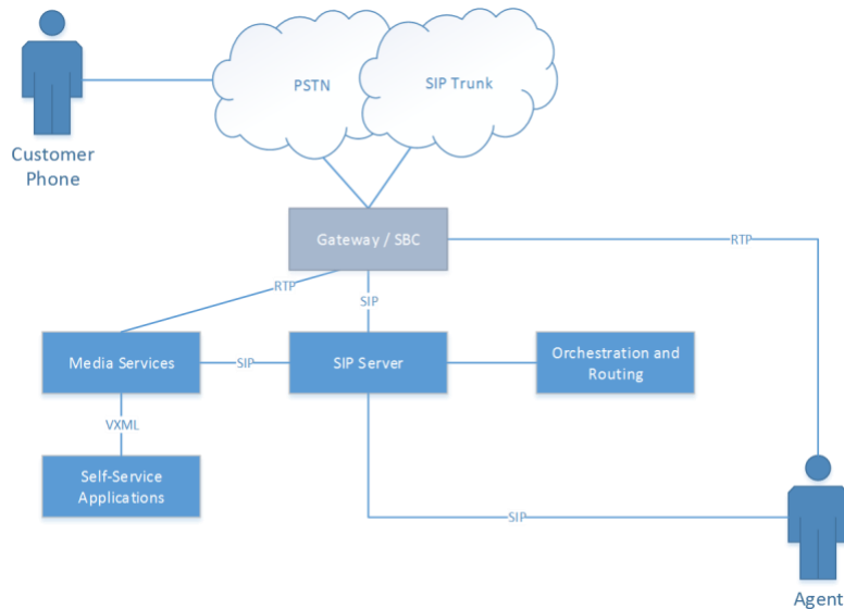
Figure 1 - SIP Solution Logical Model
