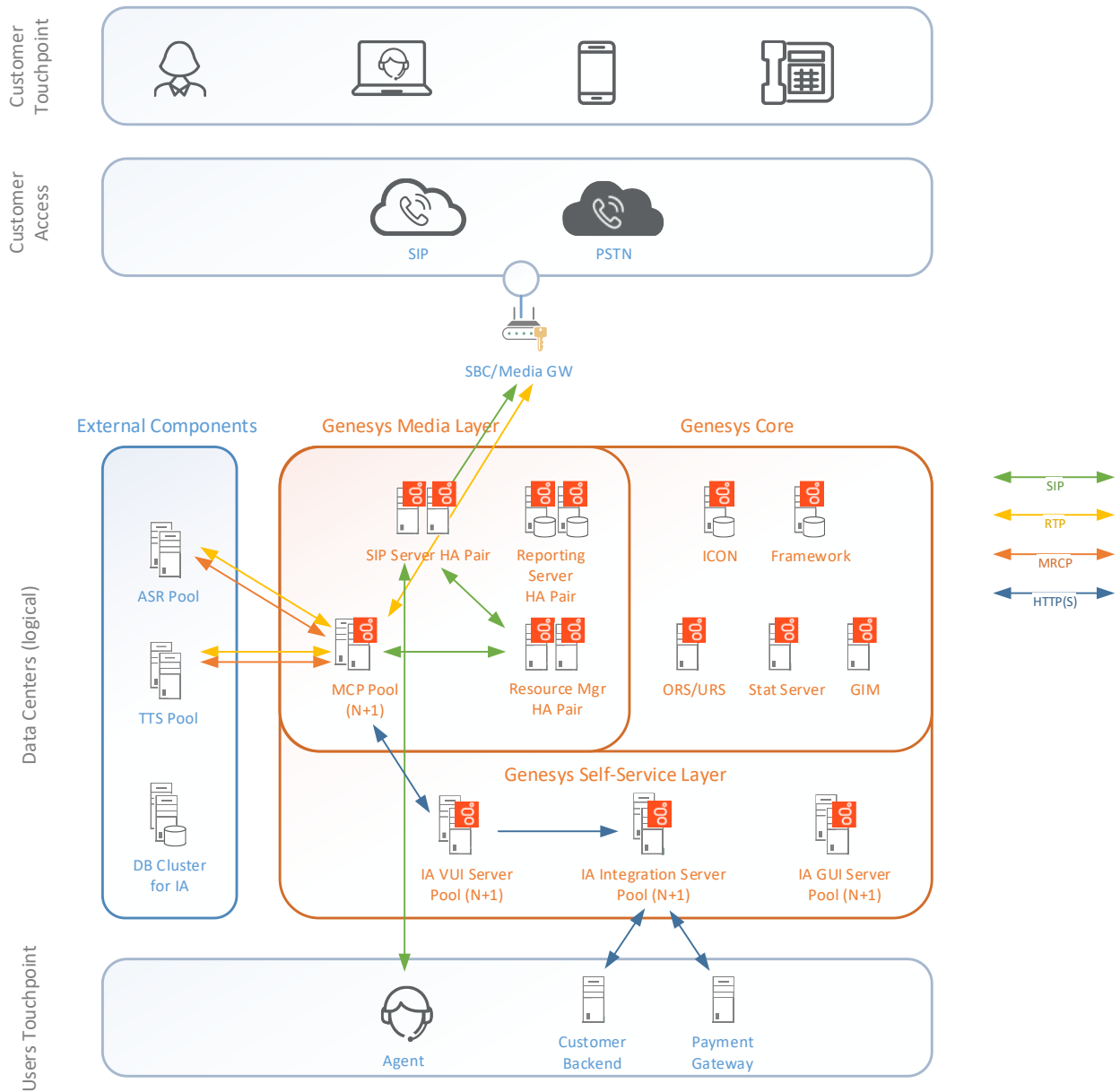
Figure 4 - High Availability Deployment Model
