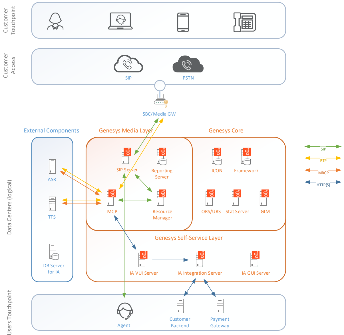
Figure 3 - Simple Deployment Model
